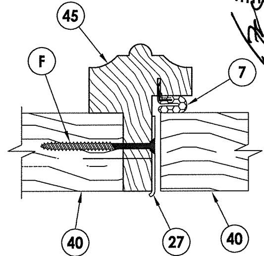
5 HORIZONTAL CROSS SECTION 3 Outswing shown (Inswing similar)
