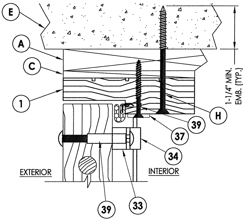
2 4 VERTICAL CROSS SECTION Outswing shown w/1X sub-buck
